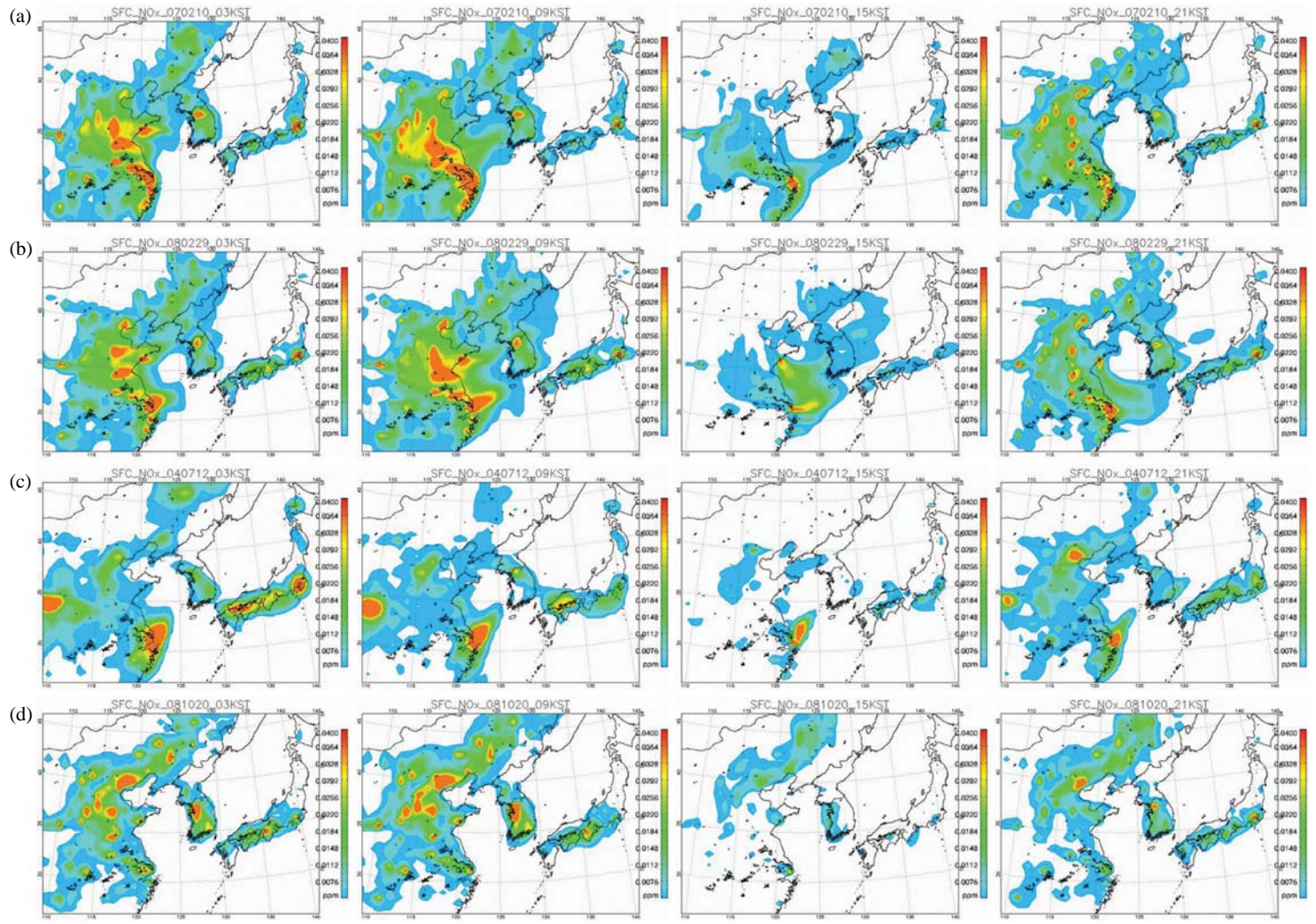
Fig. 5. The spatial distributions of surface NO x concentrations at 03, 09, 15, 21KST on (a) 10 Feb. 2007 (LRT-I case), (b) 29 Feb. 2008 (LRT-II case), (c) 12 Jul. 2004 (LRT-III case), and (d) 20 Oct. 2008 (LED case).
