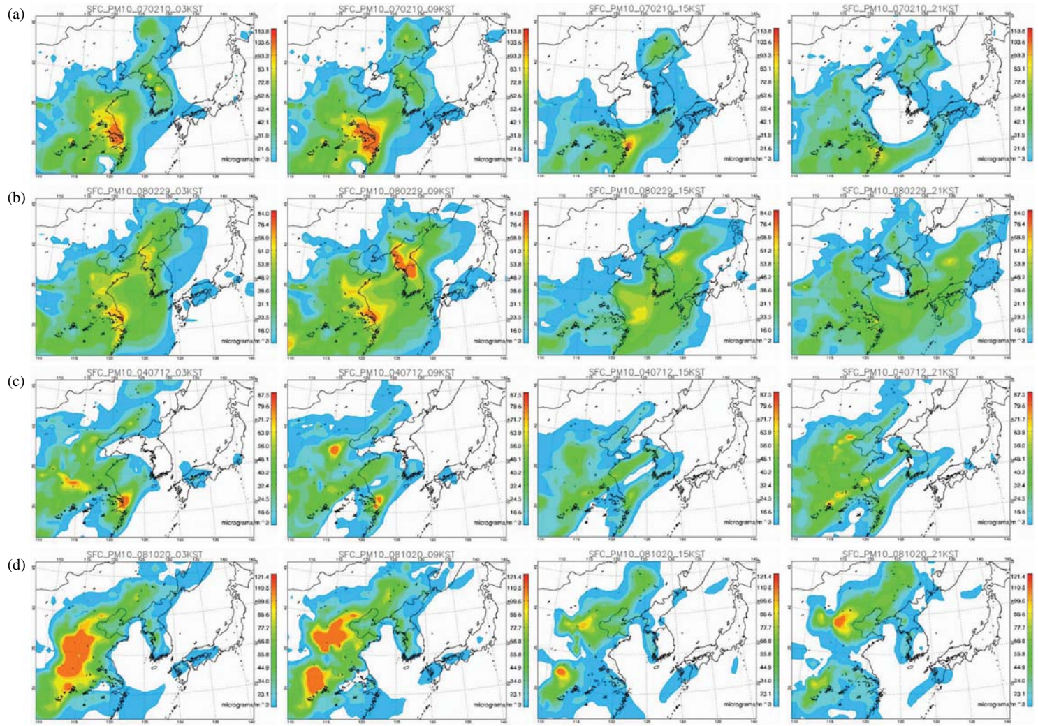
Fig. 6. The spatial distributions of surface PM 10 concentrations at 03, 09, 15, 21KST on (a) 10 Feb. 2007 (LRT-I case), (b) 29 Feb. 2008 (LRT-II case), (c) 12 Jul. 2004 (LRT-III case), and (d) 20 Oct. 2008 (LED case).
