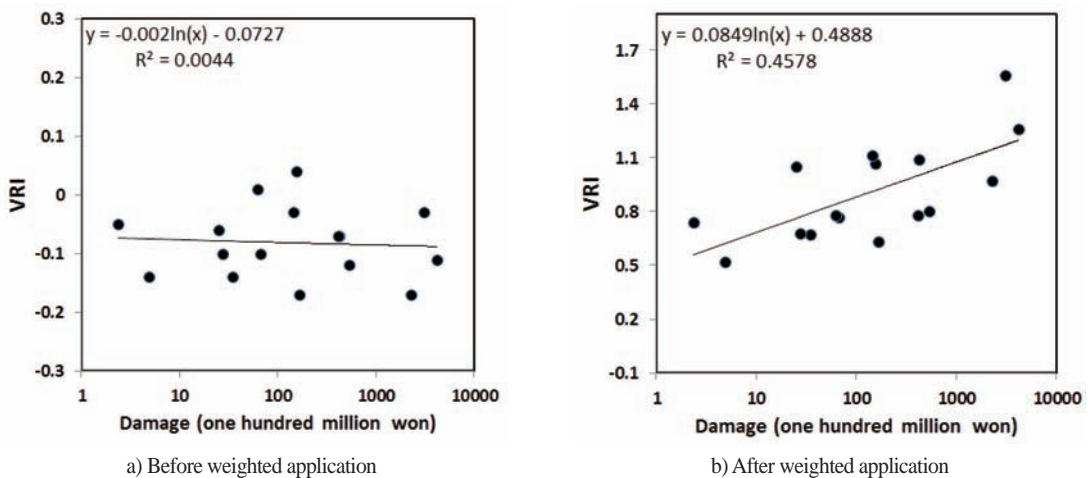
Figure 6. Scatter diagrams of damaged statistics against VRI (Vulnerability-Resilience Index) calculated a) without, and b) with applying weighting factors of climate exposure proxy variables.
