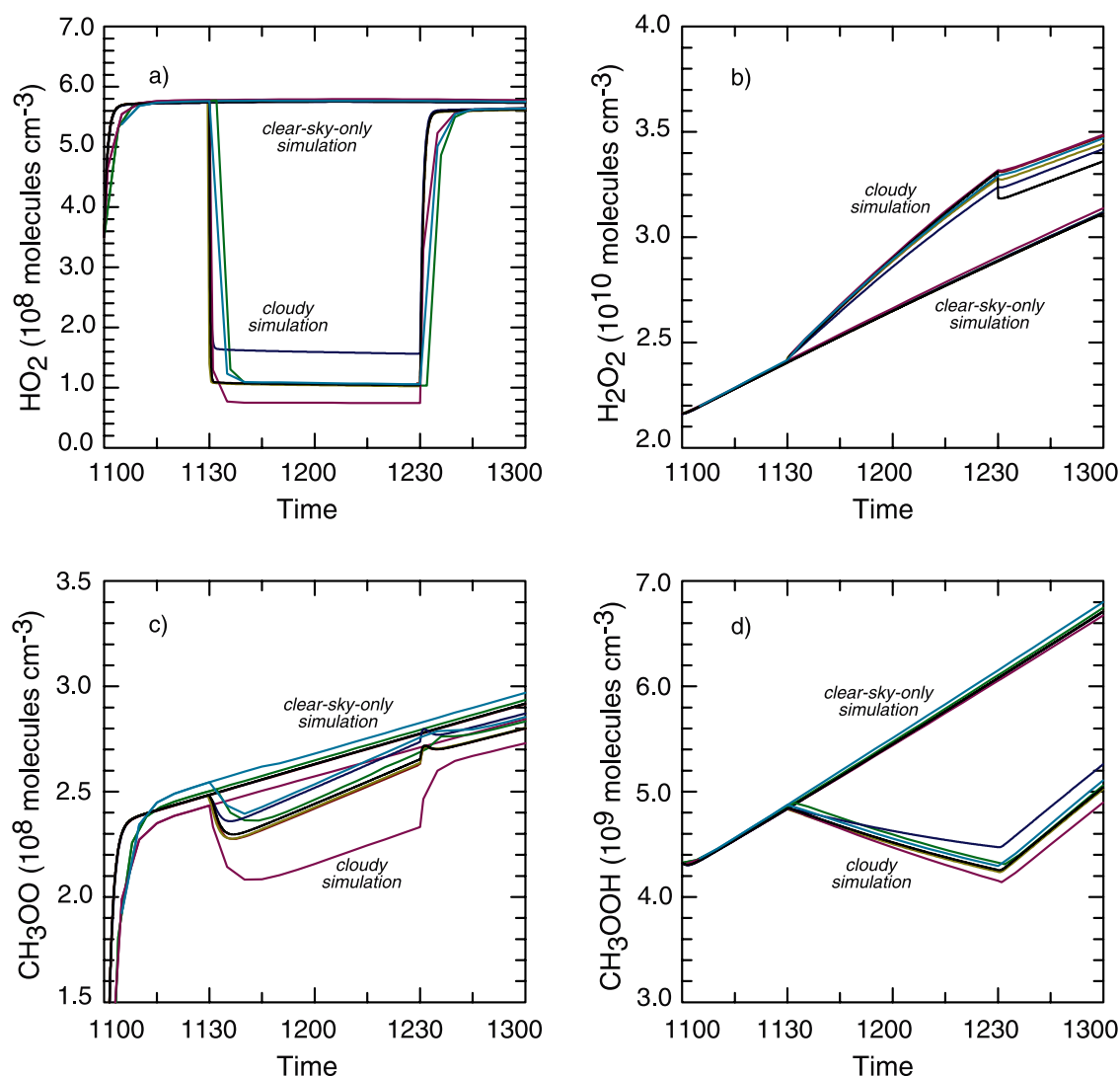
Figure 2. Total (gas + aqueous) concentration of (a) \text{HO}_2 , (b) \text{H}_2\text{O}_2 , (c) \text{CH}_3\text{OO} , and (d) \text{CH}_3\text{OOH} as a function of time for the required simulations. Color legend is shown in Figure 1.
