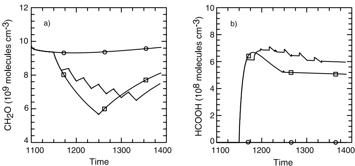
Figure 10. Total concentration of (a) \text{CH}_2\text{O} and (b) \text{HCOOH} as a function of time under constant \text{NO}_x concentrations using the Barth-Gear model for the simulation with only gas-phase chemistry (line with circles), the continuous cloudy simulation (line with squares), and the intermittent cloudy simulation (solid line).
