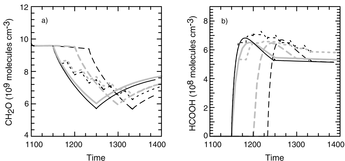
Figure 9. Total concentration of (a) \text{CH}_2\text{O} and (b) \text{HCOOH} as a function of time for the standard continuous cloud simulation (solid lines; black is the Barth-Gear model, gray the Sillman model), for the intermittent cloud simulation (dotted lines; black is the Barth-Gear model, gray the Sillman model), for the “late cloud” continuous cloud where cloud is from t = 1200 to t = 1300 (gray dashed line, Sillman model), and for the “late cloud” continuous cloud where cloud is from t = 1220 to t = 1320 (black dashed line, Barth-Gear model).
